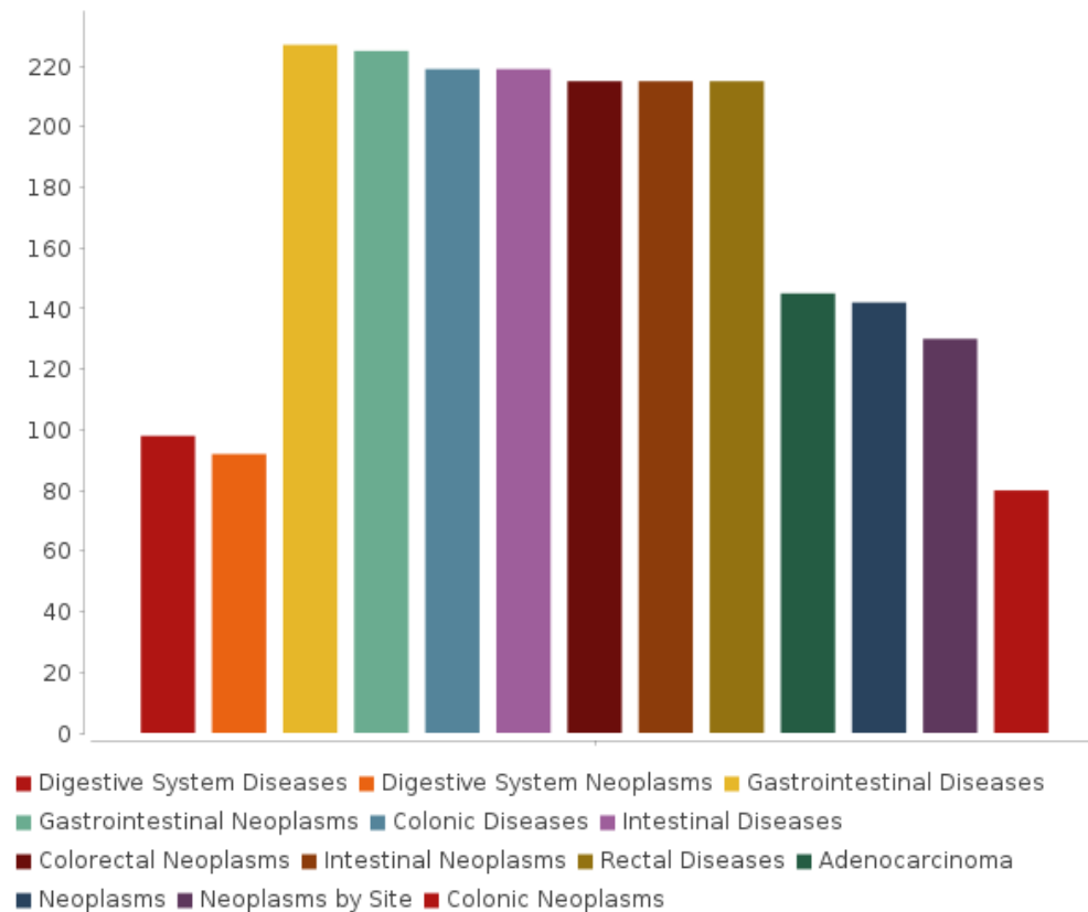
Figure 4. Enriched HumanPSD(TM) disease (2024.1) of the most frequently mutated genes in Experiment: short-term survival. The size of the bars correspond to the number of biomarkers of the given disease found among the input set.
