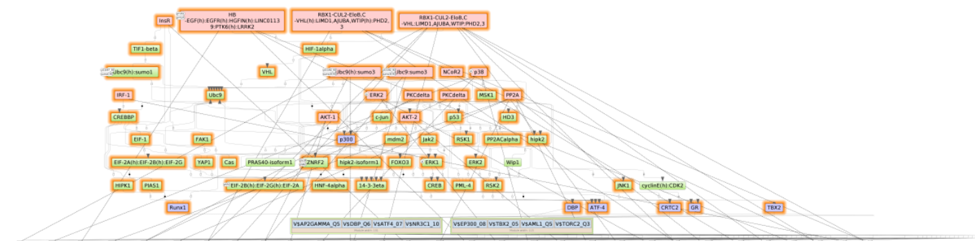
Figure 5. Diagram of intracellular regulatory signal transduction pathways of the most frequently mutated genes in Experiment: short-term survival. Master regulators are indicated by red rectangles, transcription factors are blue rectangles, and green rectangles are intermediate molecules, which have been added to the network during the search for master regulators from selected TFs. Orange frames highlight molecules presented in original mapping.
