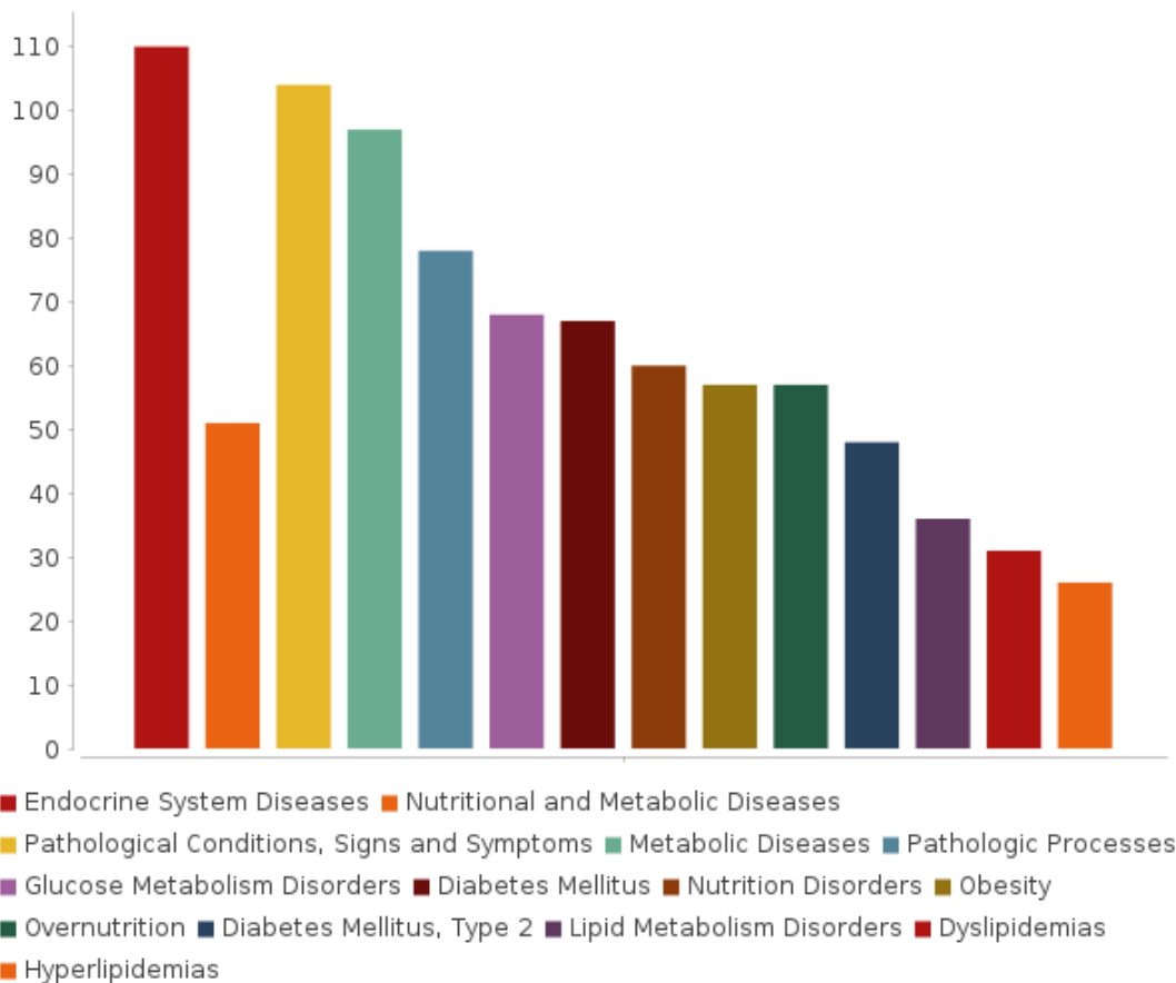
Figure 4. Enriched HumanPSD(TM) disease (2021.3) of genes carrying SNP variations in Experiment. The size of the bars correspond to the number of bio-markers of the given disease found among the input set.
