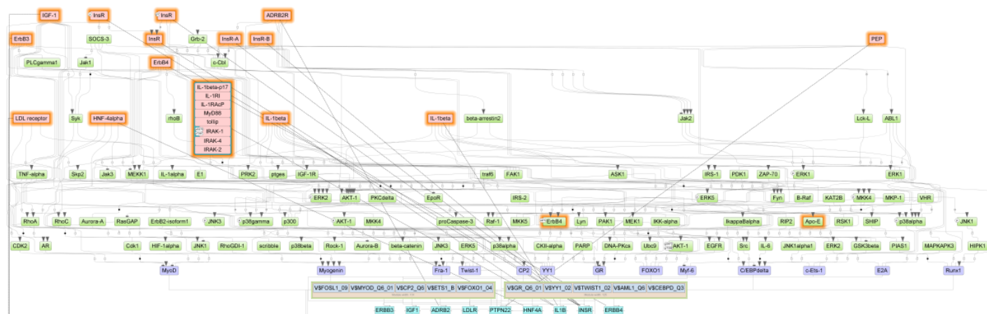
Figure 5. Diagram of intracellular regulatory signal transduction pathways of genes carrying SNP variations in Experiment. Master regulators are indicated by red rectangles, transcription factors are blue rectangles, and green rectangles are intermediate molecules, which have been added to the network during the search for master regulators from selected TFs. Orange frames highlight molecules presented in original mapping.
