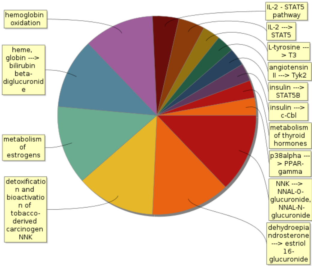
Figure 3. Enriched TRANSPATH® Pathways (2021.1) of genes carrying SNP variations in Experiment. Full classification →
