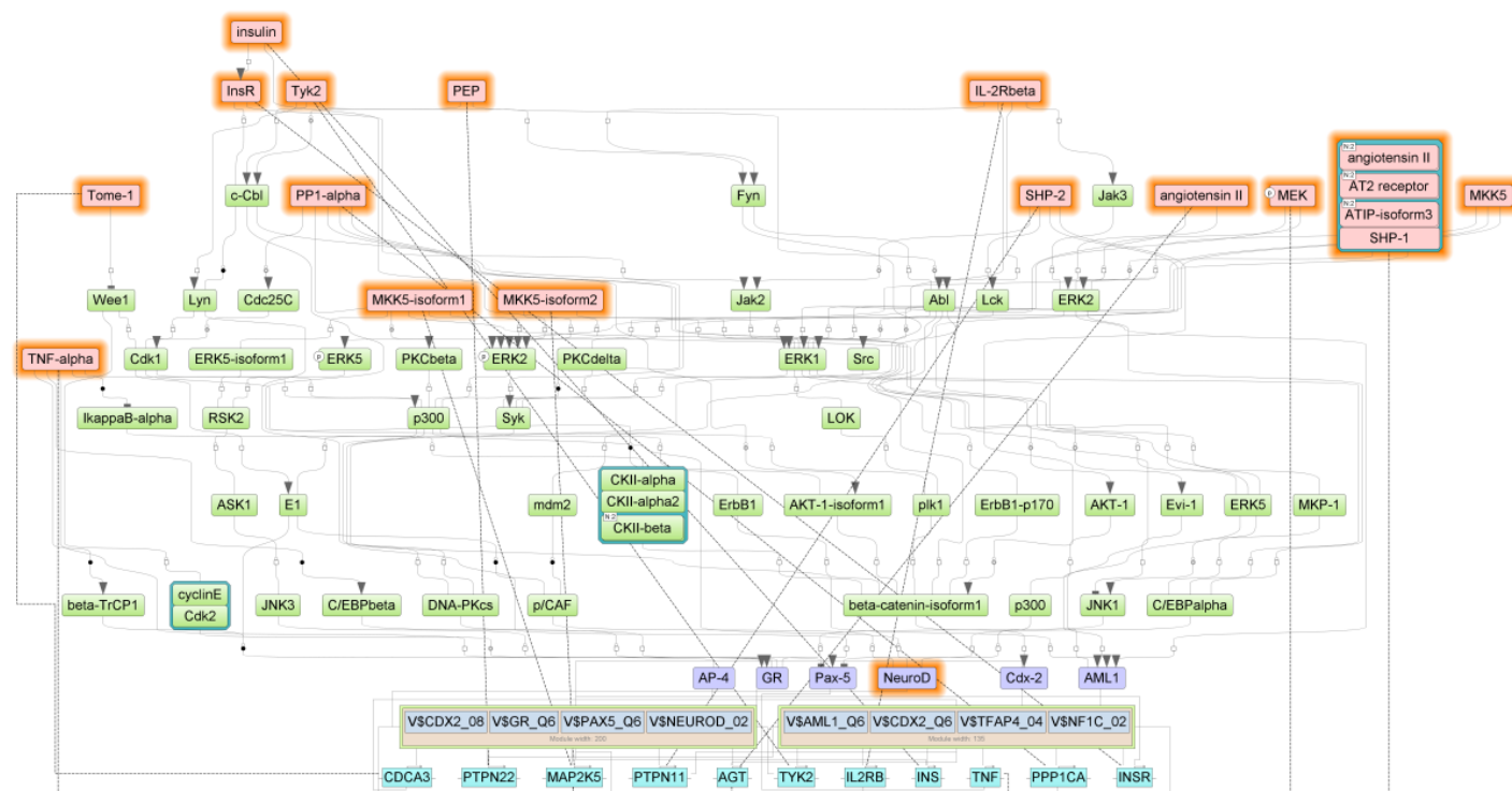
Figure 5. Diagram of intracellular regulatory signal transduction pathways of genes carrying SNP variations in Experiment. Master regulators are indicated by red rectangles, transcription factors are blue rectangles, and green rectangles are intermediate molecules, which have been added to the network during the search for master regulators from selected TFs. Orange frames highlight molecules presented in original mapping.
